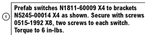
Figure 1 Mechanical Switch Assembly
